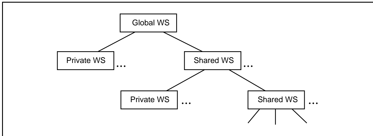
Figure 2. A workspace hierarchy.
