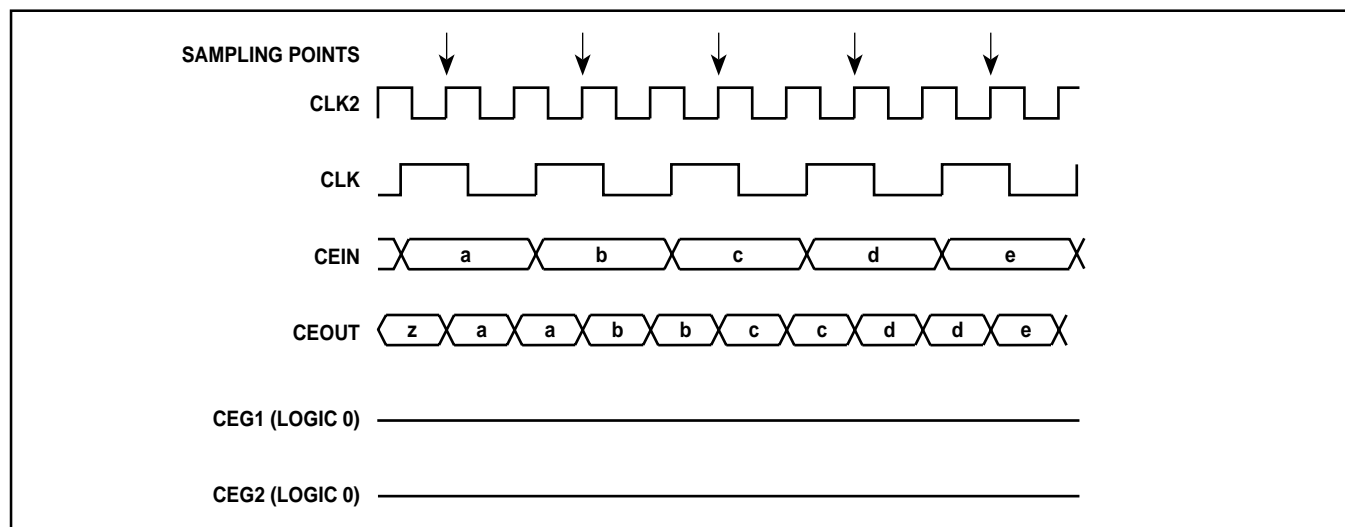
Figure 11 Convolutional encoder interface in Basic mode
