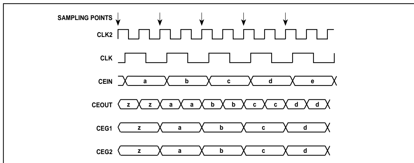
Figure 12 Convolutional encoder interface in Advanced mode
