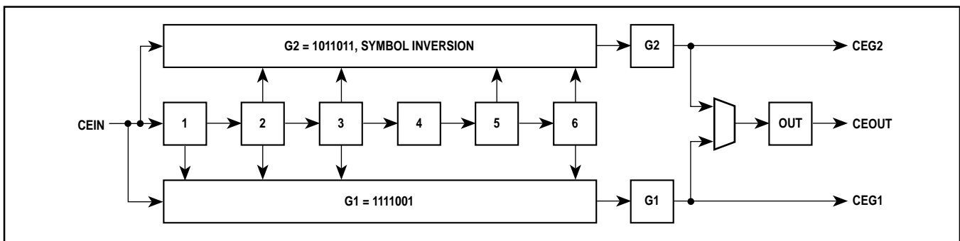
Figure 7 Block diagram of convolutional encoder
