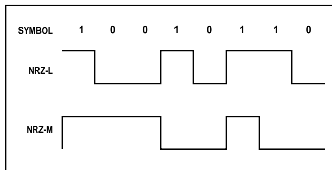
Figure 8 NRZ-L and NRZ-M waveforms
