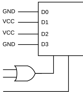
Figure 8 • Single Module CM8 Implementation
